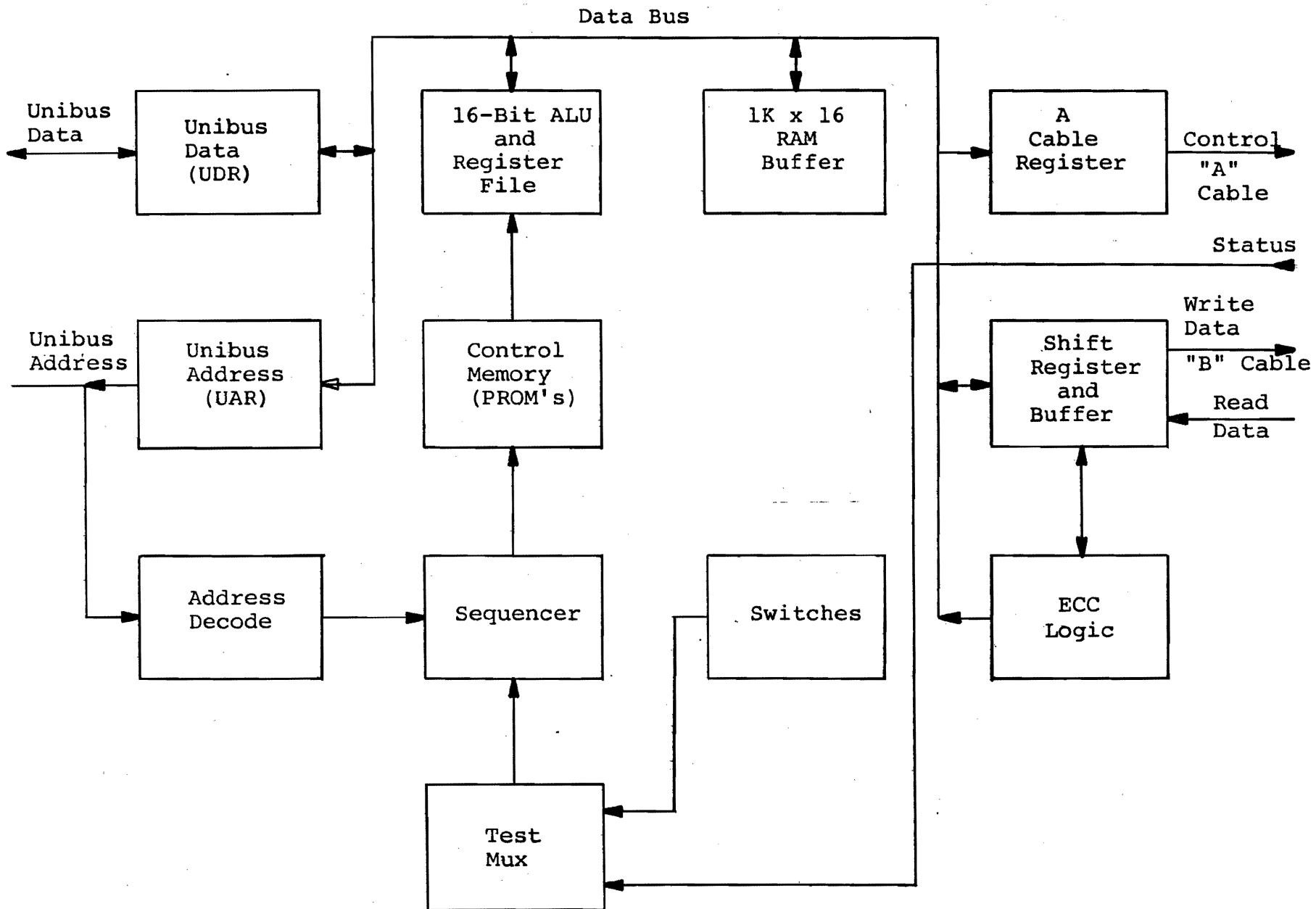
Figure 2-1 SC21 Block Diagram
