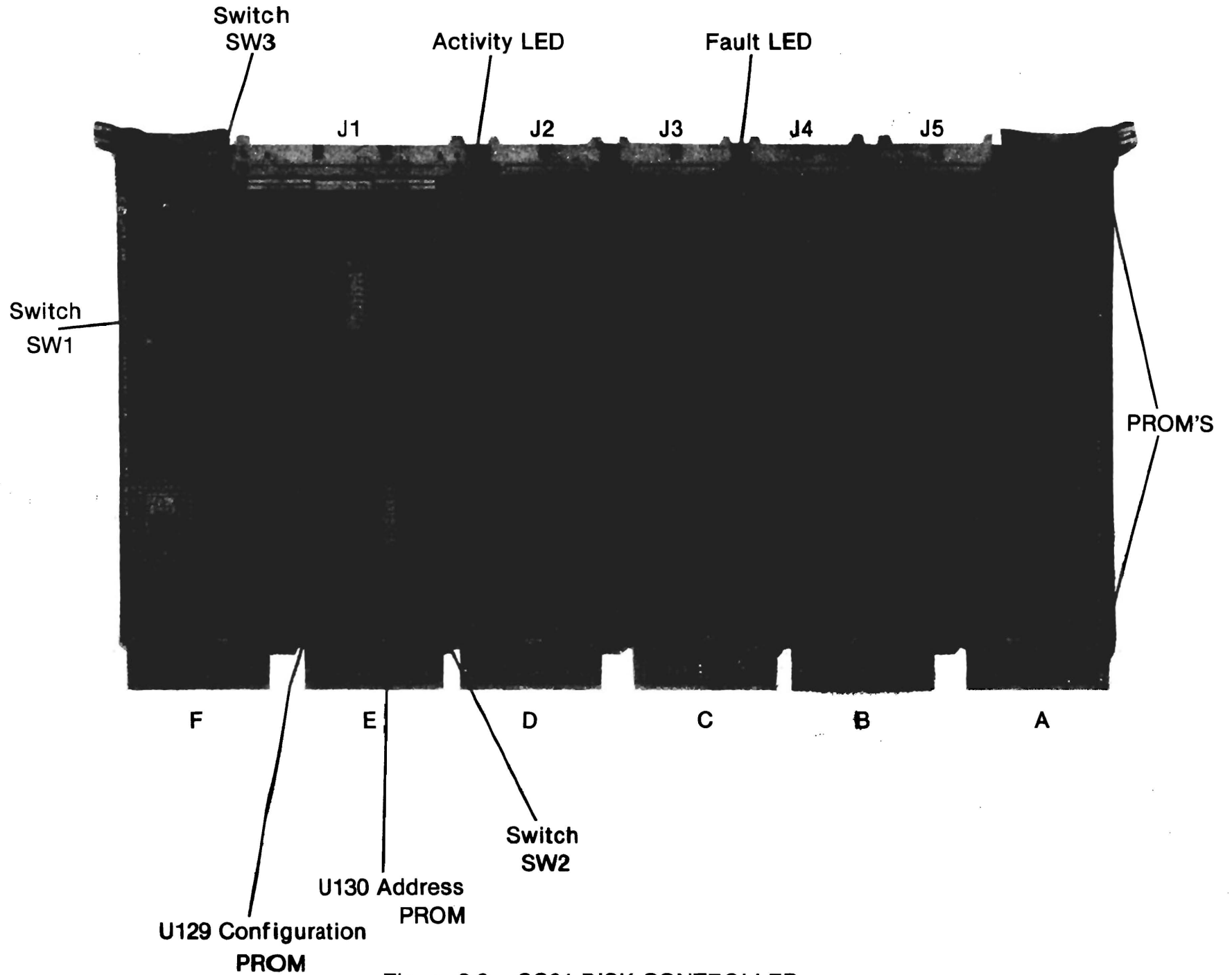
Figure 2-2 SC21 DISK CONTROLLER
