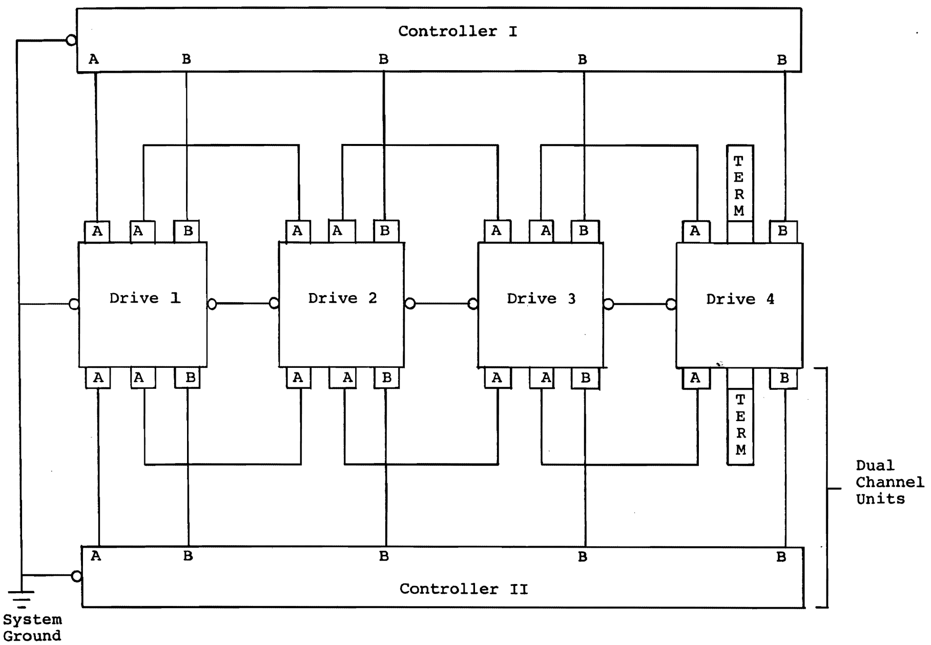
Figure 3-2 Unit Cabling
