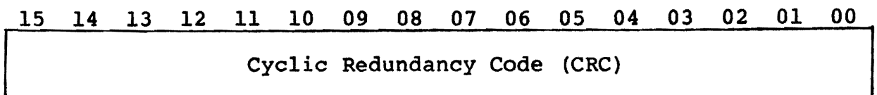
Figure 2-4 Header Format
